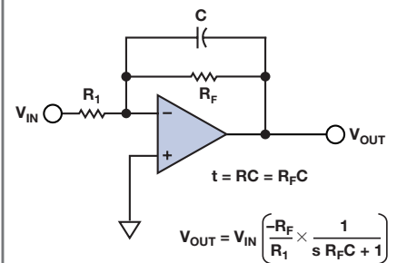
Low-Pass Filter/Integrator
