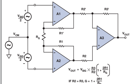
Instrumentation Amplifier
