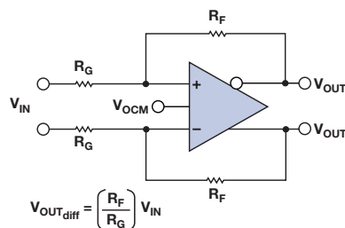
Differential Amplifier
