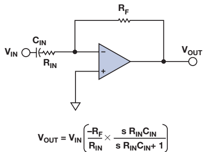
High-Pass Filter/Differentiator
